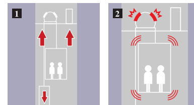
1 The car ascends at high speed. 2 Traction machine brakes safely stop the car.
